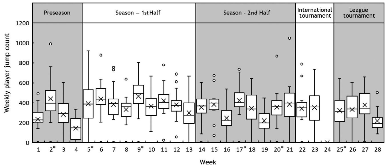
FIGURE 1 Weekly jump count variance for all players during one club season ( n = 14 players). The 6 weeks with a week-on-week increase in average player jump count of >30\% are denoted with an asterisk (*). The box represents 50% of the dataset, the ends of the box show the 1st and 3rd quartiles, whiskers extend to the furthest data point within 1.5 \times \text{IQR} from the 1st and 3rd quartiles, and circles represent data points further than 1.5 \times \text{IQR} . A horizontal line within the box signifies the median and an 'X' represents the mean
